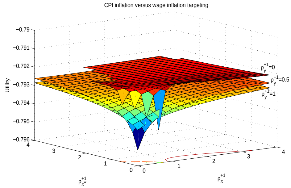
Figure 17: Period t + 1 Optimized Rules
