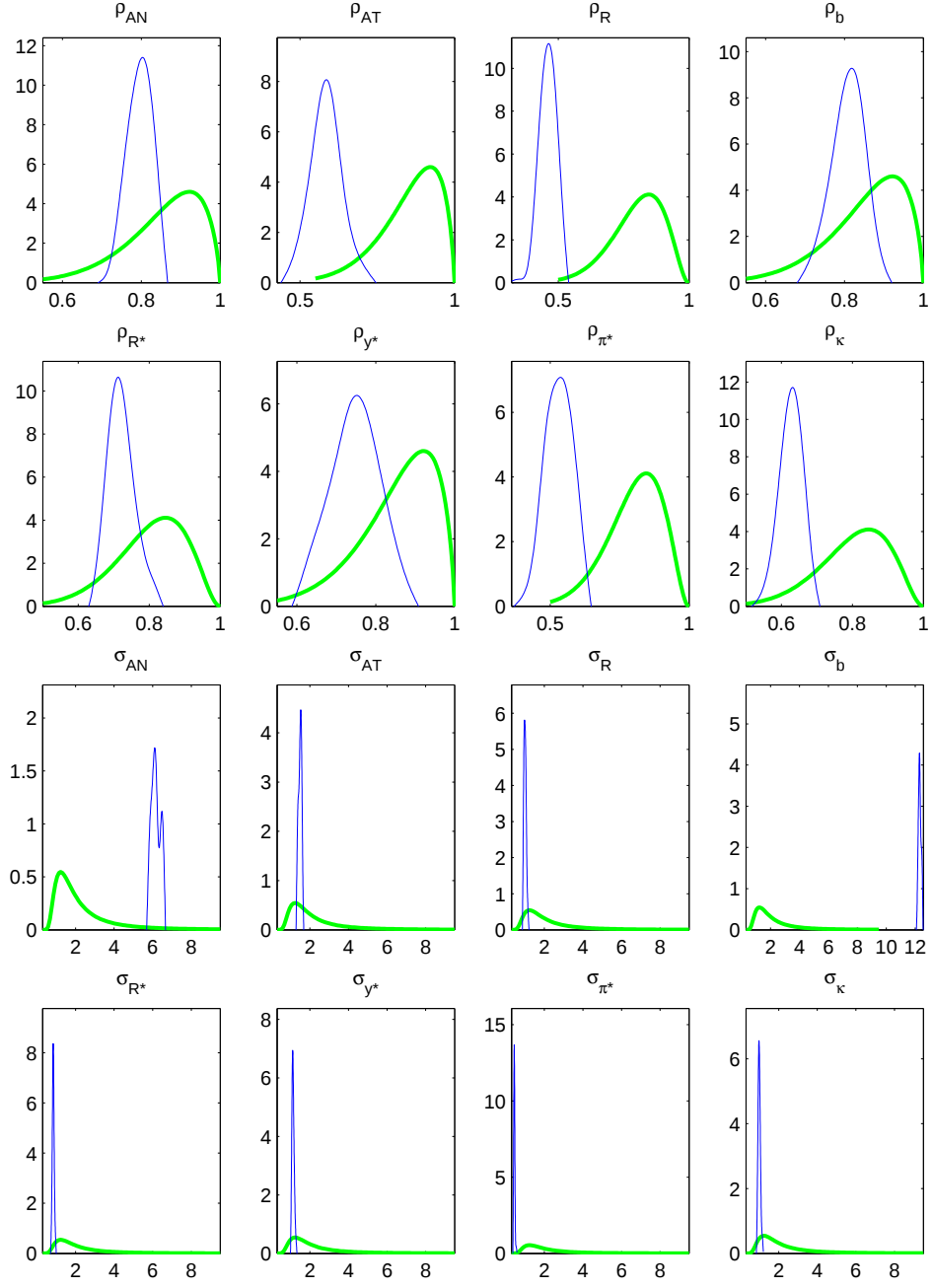
Figure 1: Prior and Posterior Distributions of the Shock Parameters
