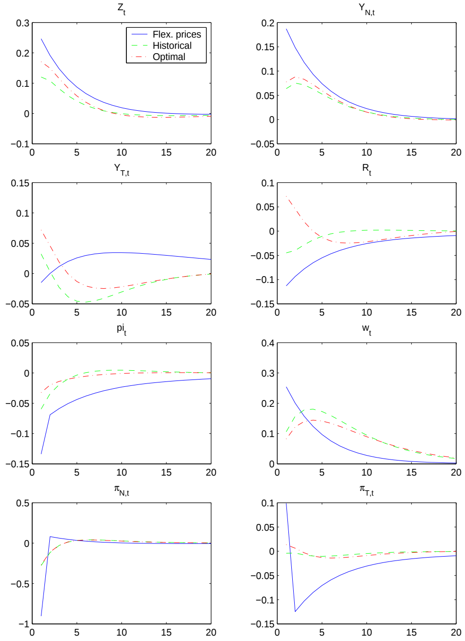
Figure 6: Non-Tradable-Goods Technology Shock
